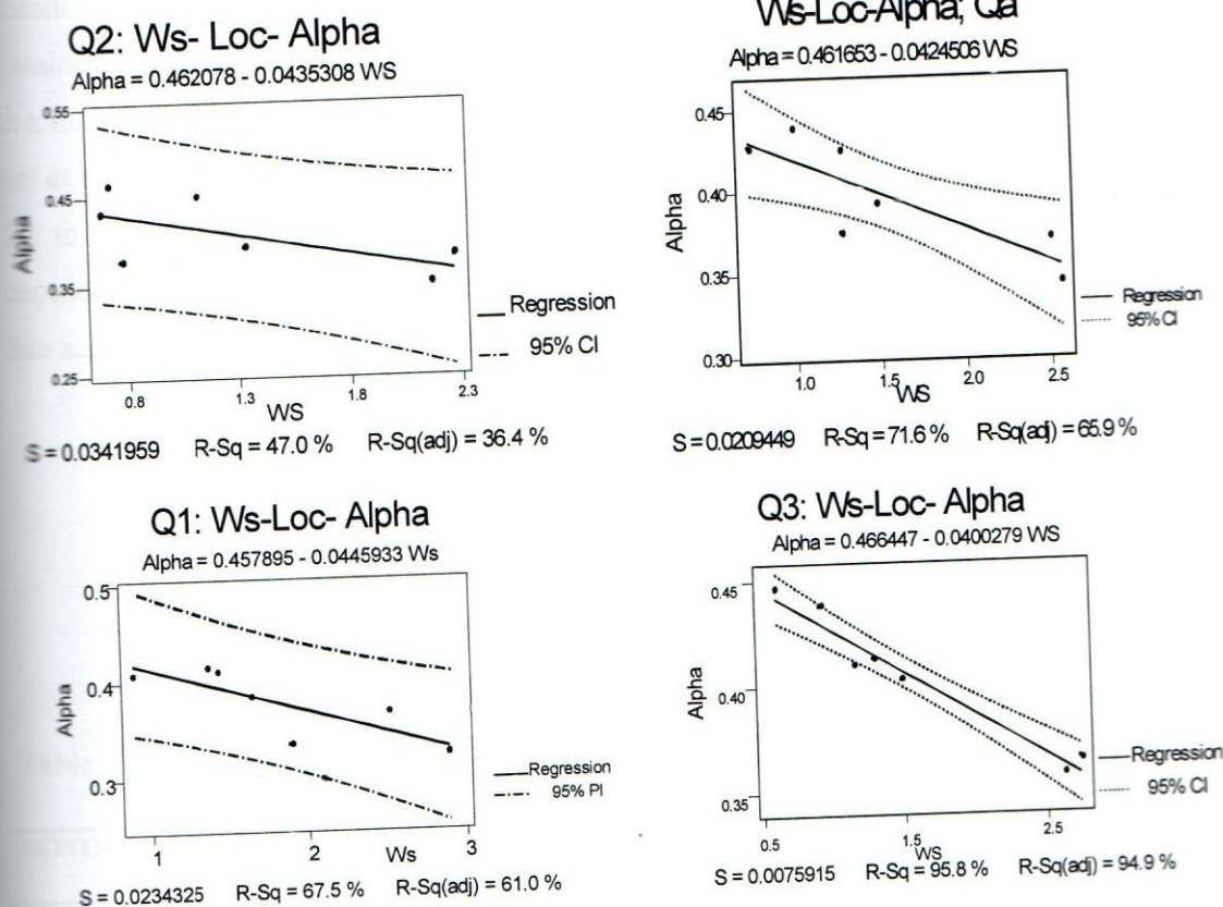
Fig: 3.10: Wind Speed Location Relationship for Lake Shore (LS) stations.
