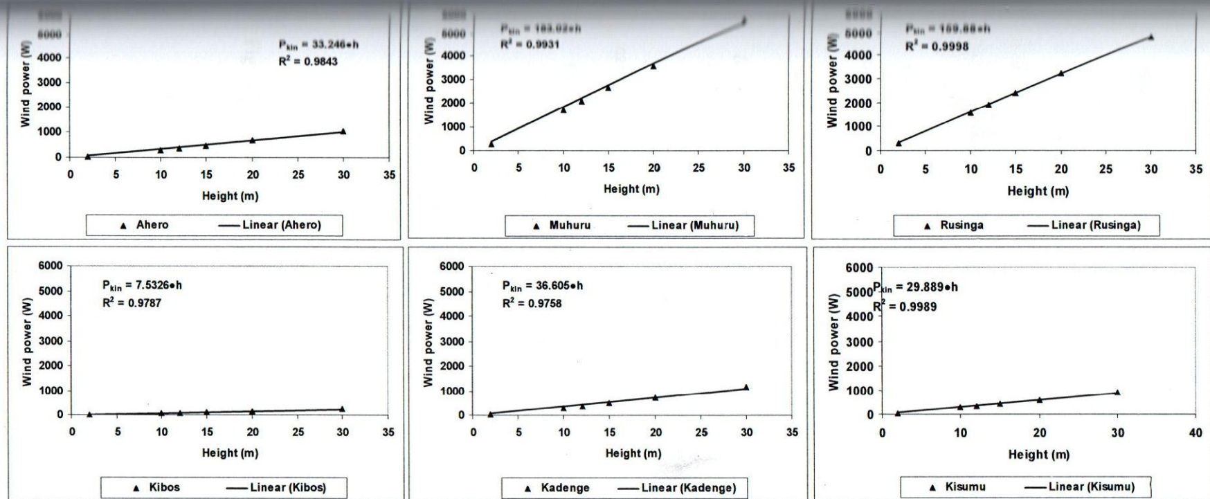
Fig.B3.13 Wind Energy Power potential with Height for 6 LS Stations.
