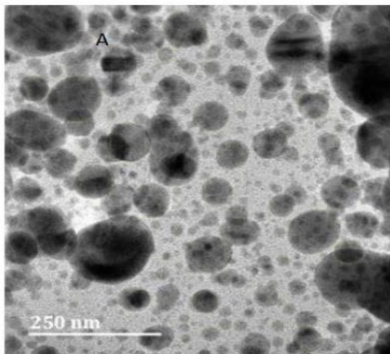
Figure 57 A: TEM micrograph dichloromethane-ethyl acetate-Ag NPs
