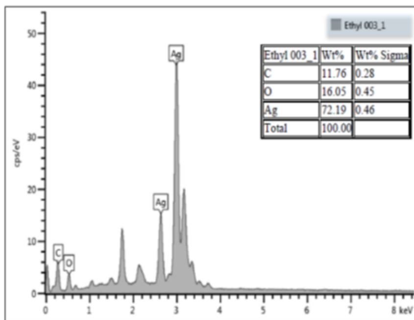
Figure 49: EDX micrograph ethyl acetate-Ag NPs
