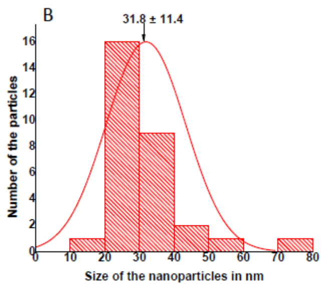
Figure 56 B: Particle size distribution histogram of methanol-Ag NPs
