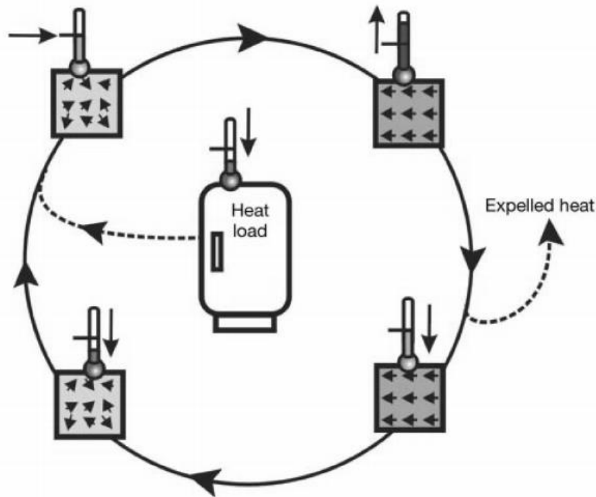
Figure 2. 2: Magnetic-refrigeration cycle
