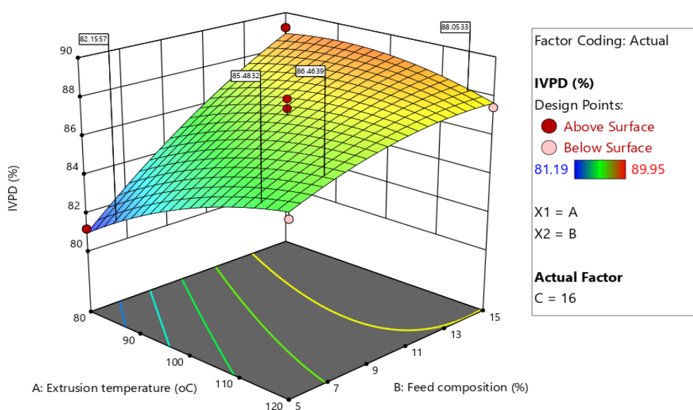
Figure 6.3. The 3D surface plot for the effect of extrusion temperature and feed composition on in vitro protein digestibility of extruded flour at constant feed moisture of 16%.
