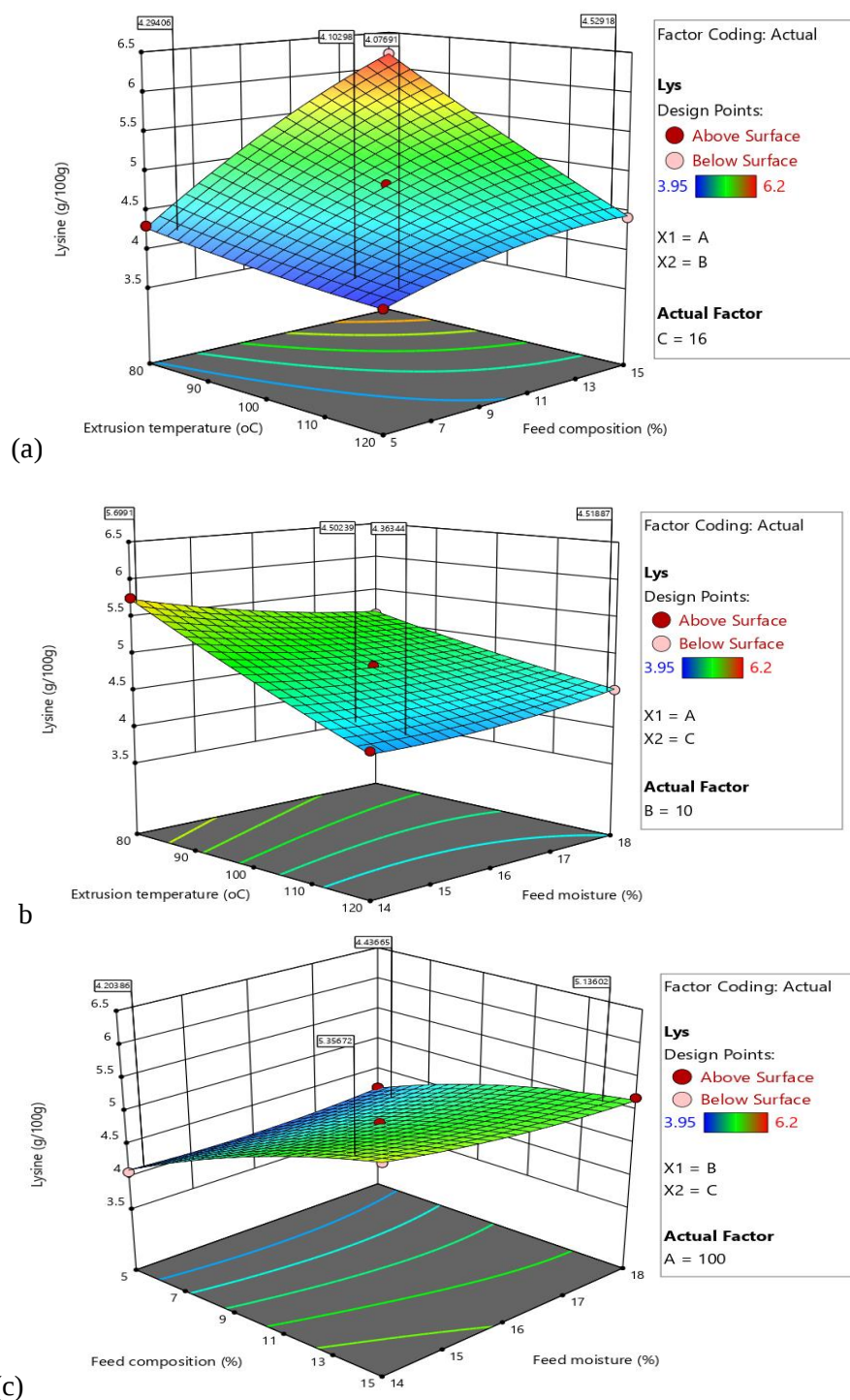
Figure 5.3. The 3D surface plots show the effects of extrusion temperature, feed composition and feed moisture on the lysine content of maize-cassava leaf instant flour. (a) Feed moisture was held constant at 16% (b) Feed composition was held constant at 10% (c) Extrusion temperature was held constant at 100°C.
